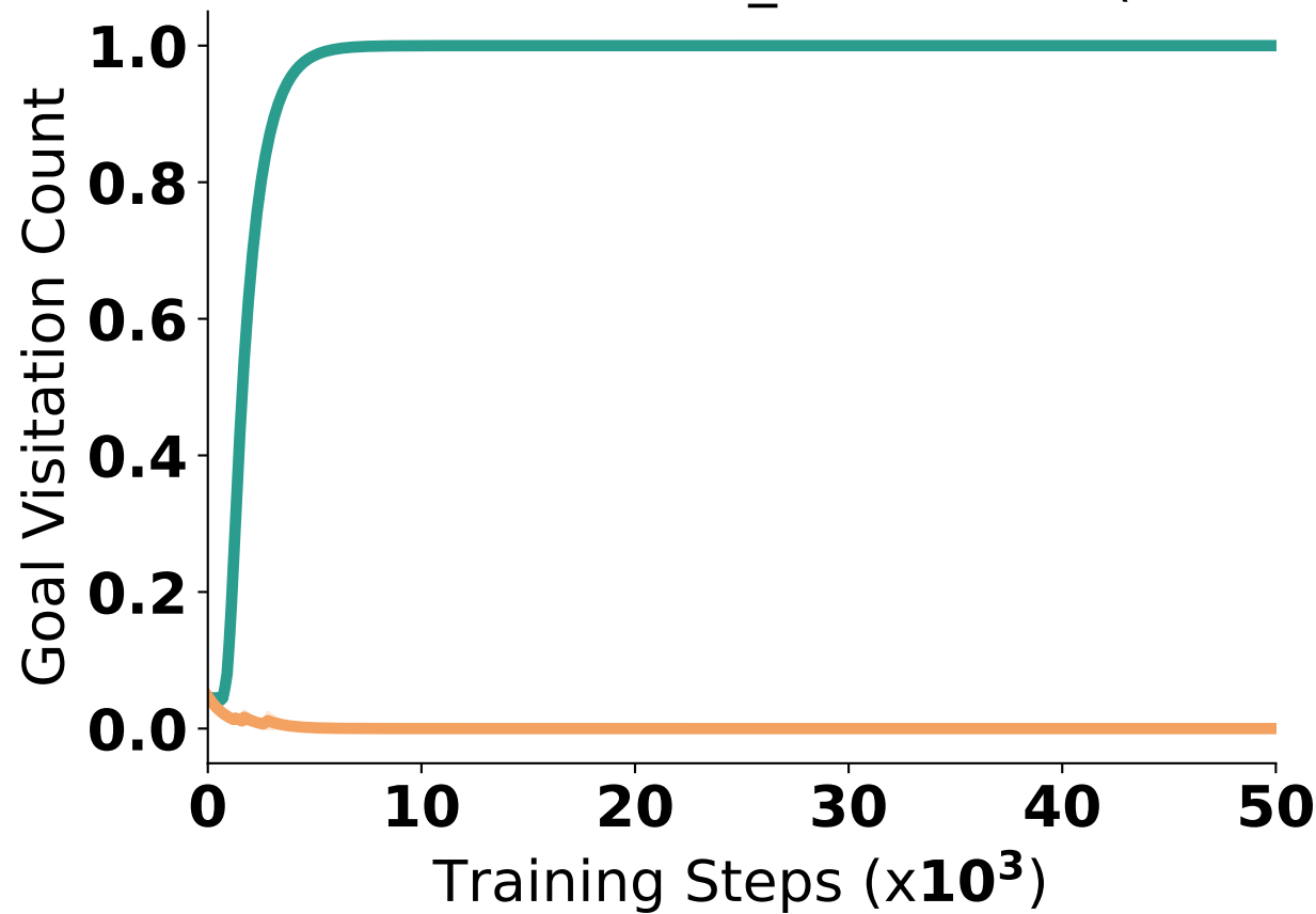
Gridworld-Bottleneck_FullRandom(80.0%)
